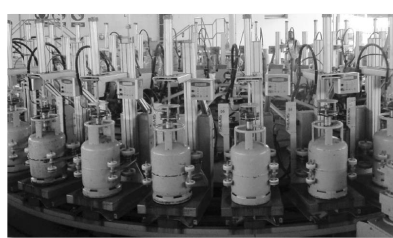
LPG Elektronical Carousel Refilling Cylinder
